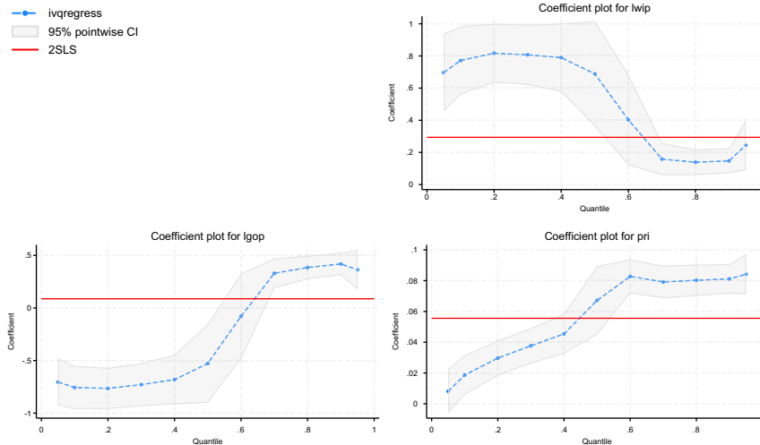
Figure 2. Smoothed instrumental variable quantile regression.
