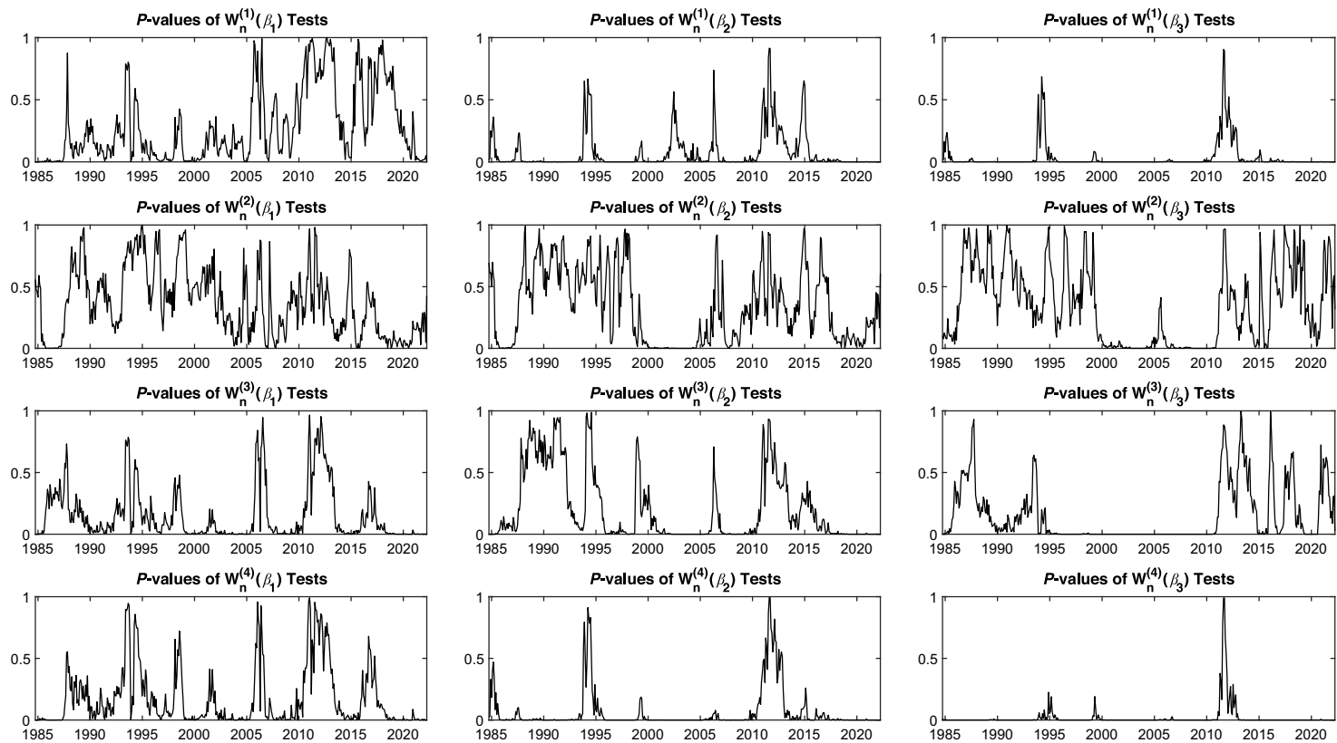
Figure C1. p -values of Wald statistics using rolling estimation.
