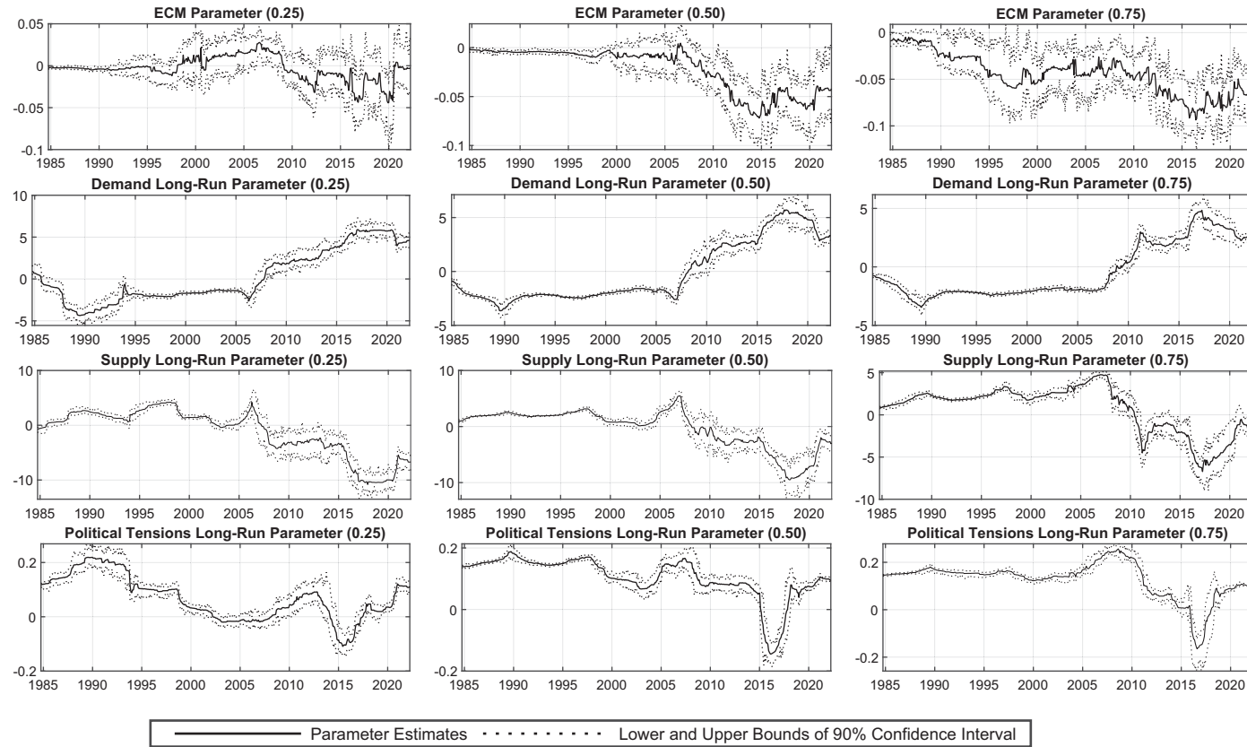
Figure 3. Time-varying QARDL error-correction model.
