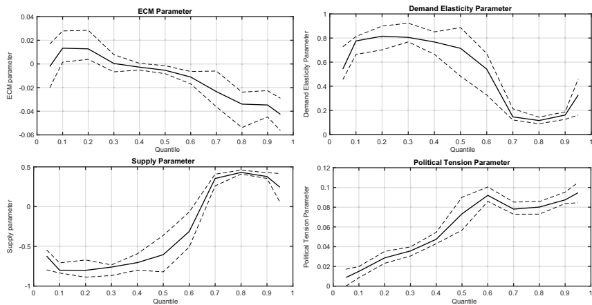
Figure 1. QARDL error-correction model.
