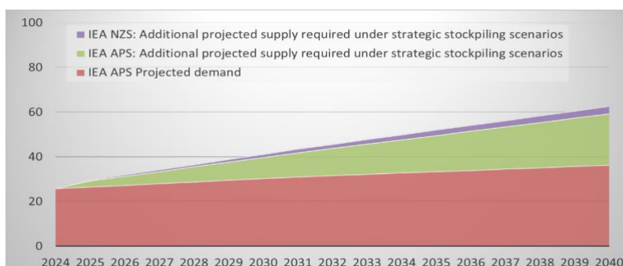
Fig. 5 | Projected supply requirements for copper under IEA APS and NZS, including global strategic stockpile accumulation. This figure illustrates the projected supply trajectory for copper under the IEA’s APS pathway, together with the additional supply requirements generated by the inclusion of strategic stockpiling under both the APS and NZS. The red area represents baseline supply required under APS, while the green and purple areas reflect the additional supply needed to build strategic reserves under APS and NZS, respectively.
