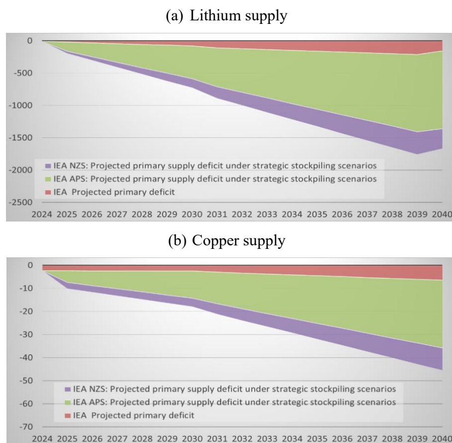
Fig. 6 | IEA current, APS, and NZS scenarios of supply shortfall of lithium and copper including global strategic stockpile. This figure projects supply-demand imbalances for lithium (top panel) and copper (bottom panel) under three IEA scenarios: the base demand, APS, and NZS, each adjusted to include global strategic stockpiling requirements. The red area represents baseline primary deficit required under APS, while the green and purple areas reflect the additional deficit if strategic reserves are built under APS and NZS, respectively.
